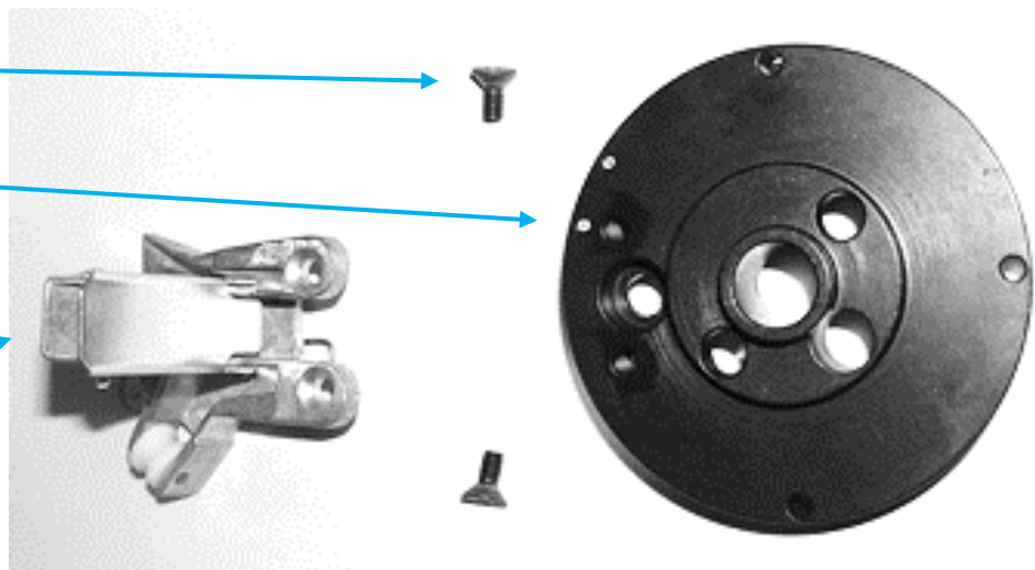
Flat Socket Head Mounting Screws (2)
