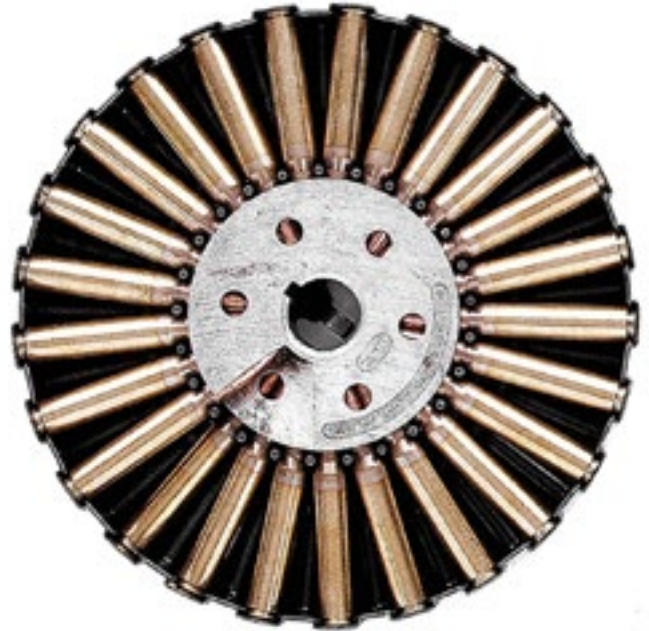
This photo shows the layout of the inside of a Lewis 47-round rotary magazine, loaded with .30-06 cartridges.
